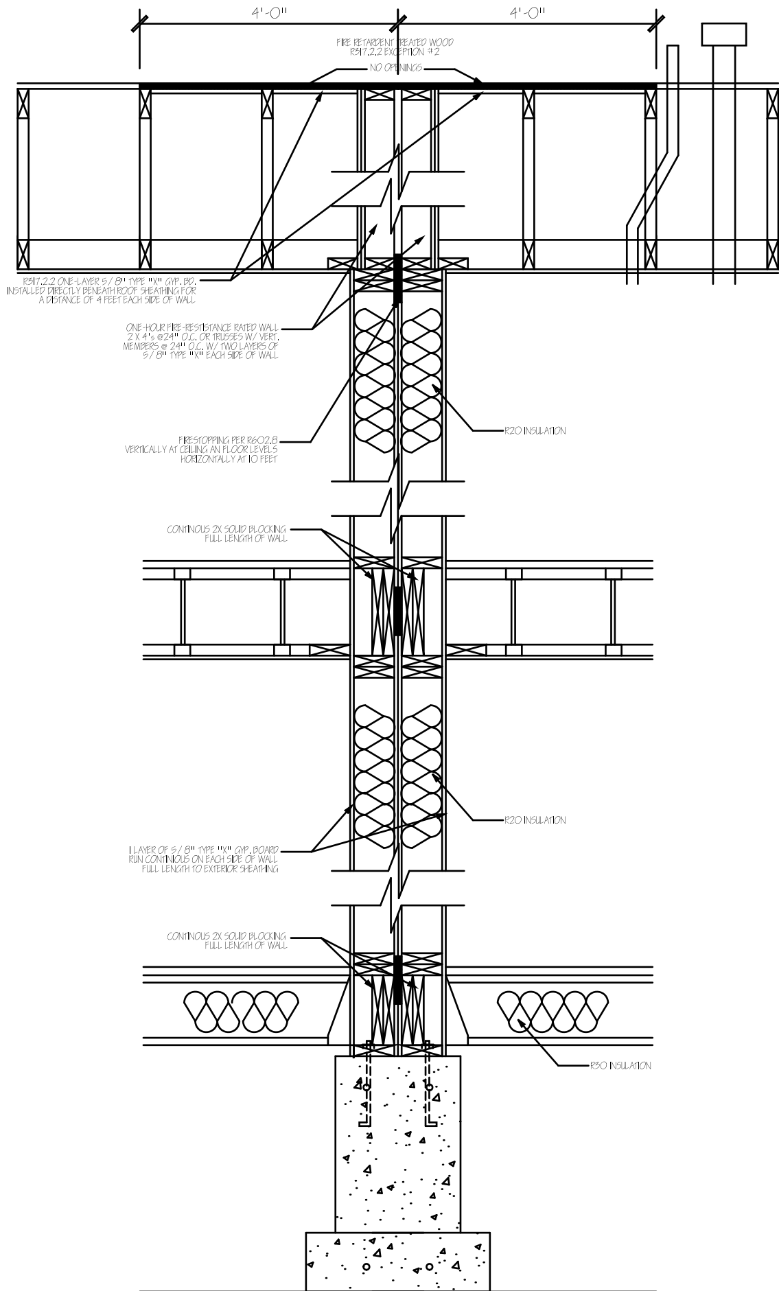
TOWNHOUSE WALL DETAIL
